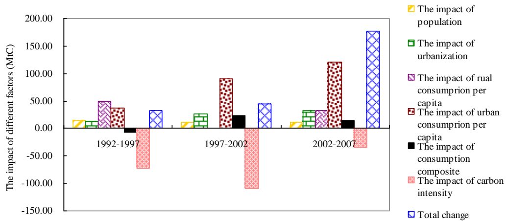
Fig. 6 The impact of different factors on indirect carbon emissions
