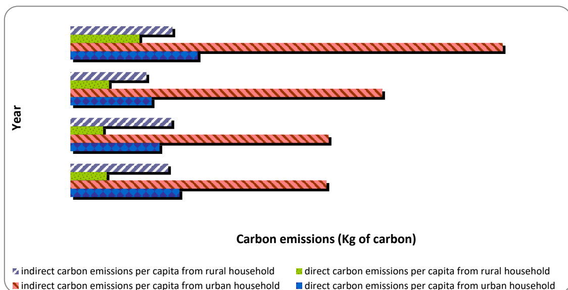
Fig.2 CO 2 emissions per capita from household consumption
