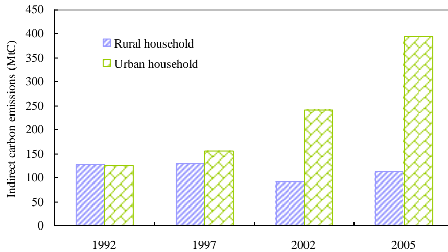
Fig. 5 The indirect carbon emissions from household consumption
