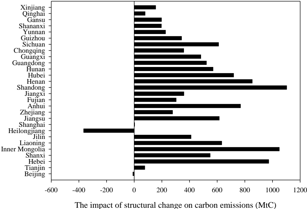
Fig. 7 The impact of economic structural change on provincial carbon emissions
