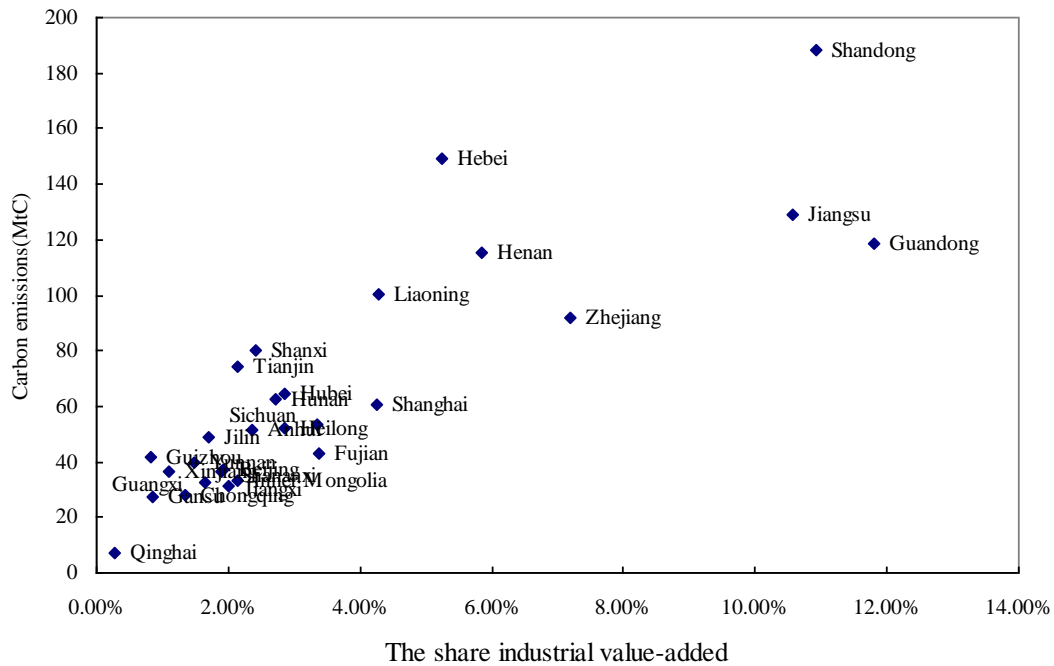
Fig. 2 Carbon emissions and the share of industrial value-added in 2007
