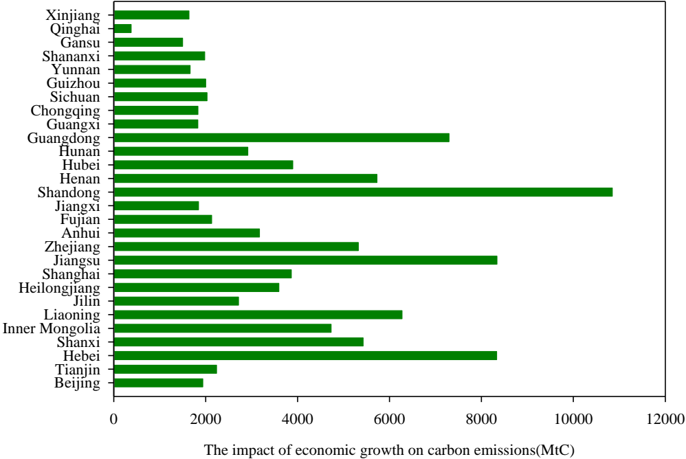
Fig. 6 The impact of economic growth on provincial carbon emissions
