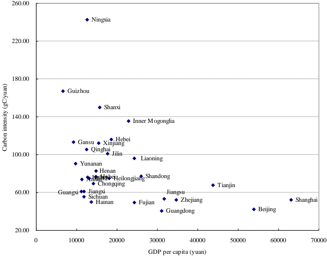
Fig. 5 Provincial carbon intensity and GDP per capita in 2007
