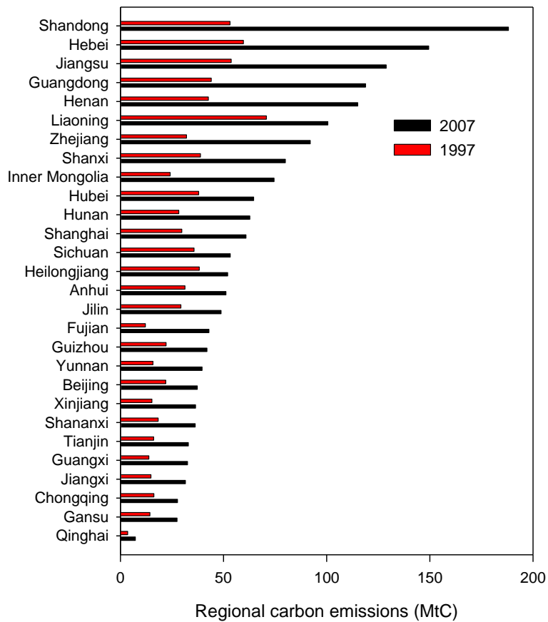
Fig. 1 Provincial carbon emissions in 1997 and 2007
