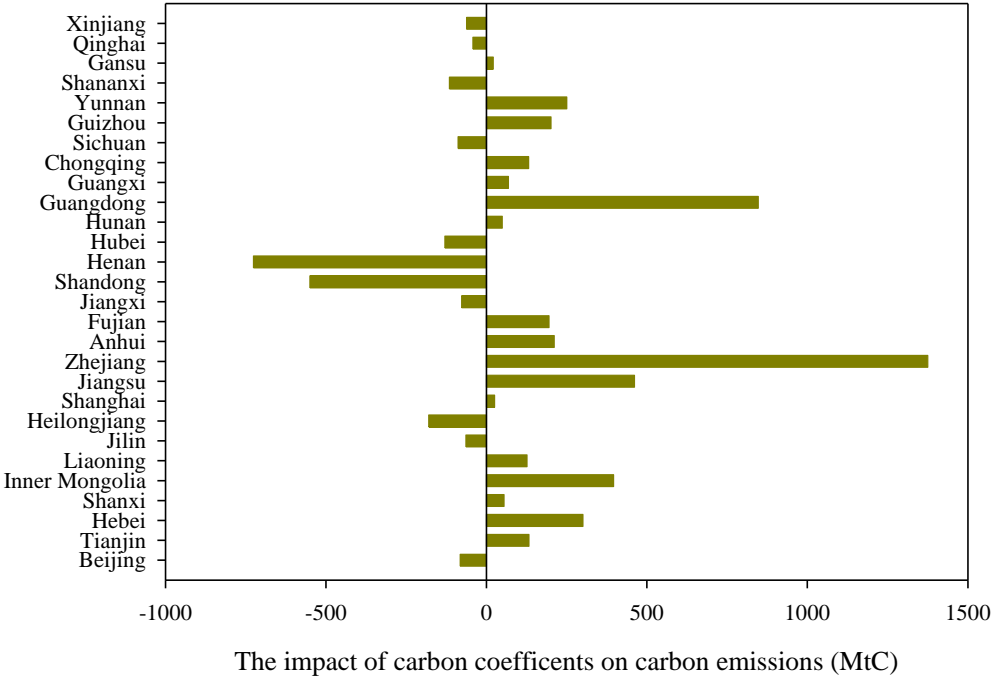
Fig. 9 The impact of carbon coefficients on provincial carbon emissions
