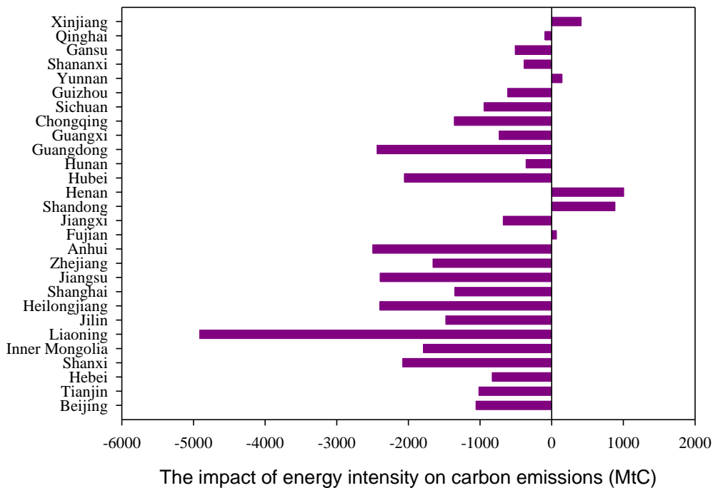
Fig. 8 The impact of energy intensity on provincial carbon emissions
