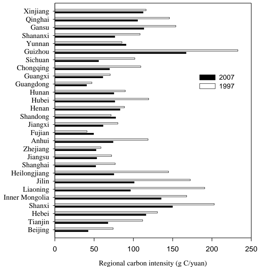
Fig. 4 Provincial carbon intensity in 1997 and 2007
