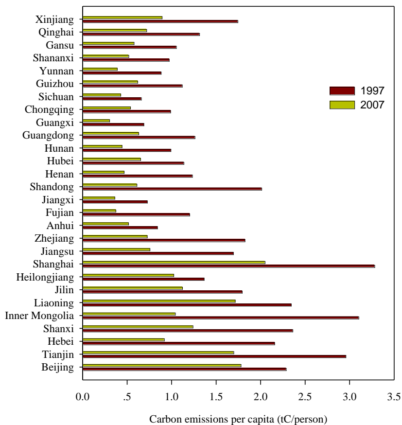
Fig. 3 Provincial carbon emissions per capita in 1997 and 2007
