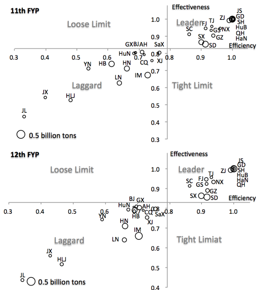
Figure 7 Strategic positions in terms of CO 2 emissions reduction performance
